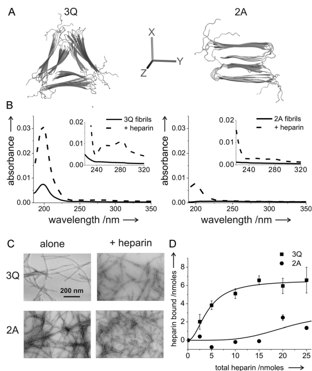
Figure 1. Binding of heparin to fibrils of A \beta_{1-40} with different morphology. A) Models of the 3Q (left) and 2A (right) fibrils viewed down the fibril long axis Z. [9] Each model comprises six layers of hydrogen-bonded peptides produced using coordinate pdb files, from Dr. Robert Tycko, with flexible N-terminal residues (not restrained by NMR data) added. B) Flow LD spectroscopy of 3Q (left) and 2A (right) fibrils (0.9 mg mL -1 ) in the absence or presence of a fivefold mass excess of 5 kDa heparin. Samples were diluted 20-fold to reduce absorbance at lower wavelengths. Insets show long-wavelength LD spectra of undiluted fibrils in the absence or presence of a fivefold mass excess of 5 kDa heparin. C) TEM images of 3Q (top) and 2A fibrils (bottom). Fibrils were grown alone or with a fivefold mass excess of 5 kDa heparin added during fibril formation. Scale bar is 200 nm in all images. D) Heparin binding to 3Q (■) and 2A fibrils (●). Results shown as mean \pm standard error of the mean (S.E.) from experiments carried out in triplicate. Data were analyzed using nonlinear regression fitted using the Hill equation (solid lines). The fibrils were suspended at 0.9 mg mL -1 before sedimentation.
